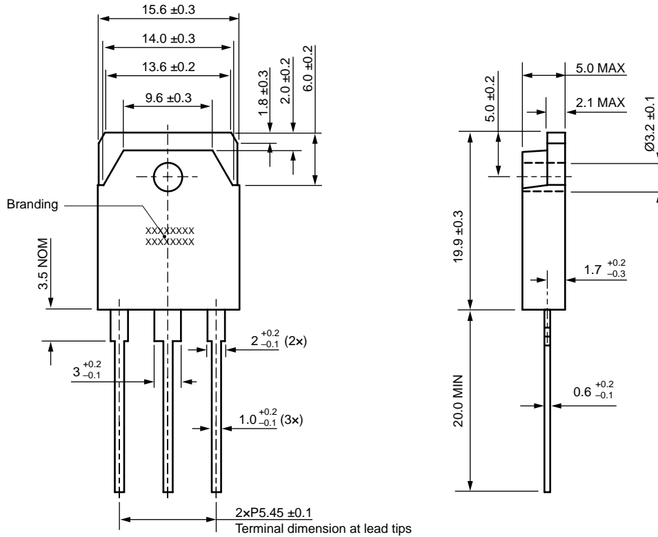
PACKAGE OUTLINE DRAWING, TO-3P
